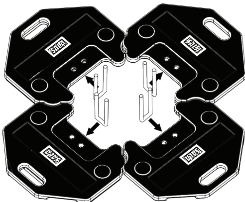
Figure 7 - Lay Out Base Weights and U-Bolts
