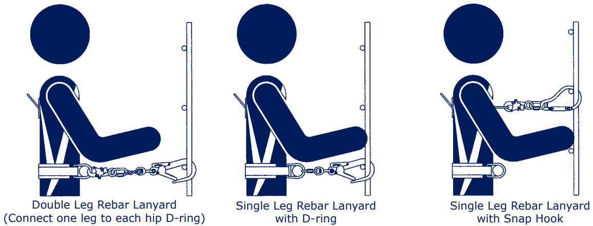
Figure 5 - Connecting To Your Body Support
