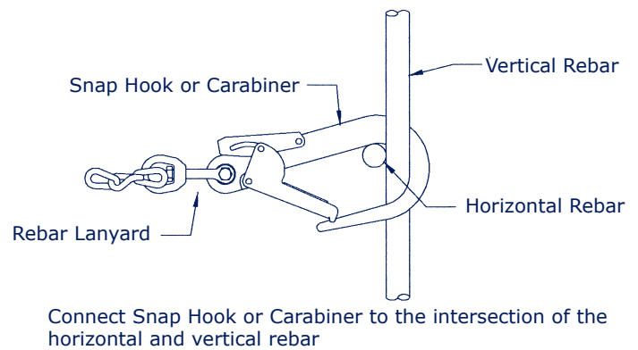
Figure 6 - Connecting To The Anchorage
