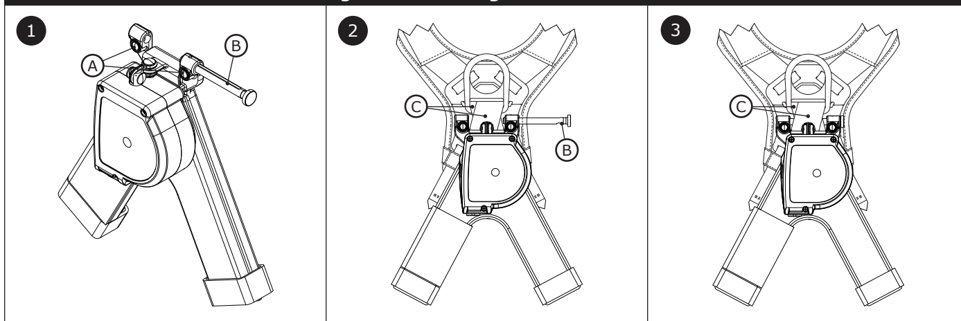
Figure 10A - Straight-Pin Interface
