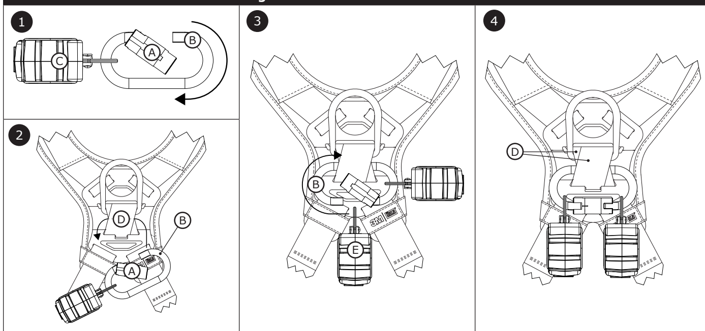
Figure 10B - Carabiner Interface
